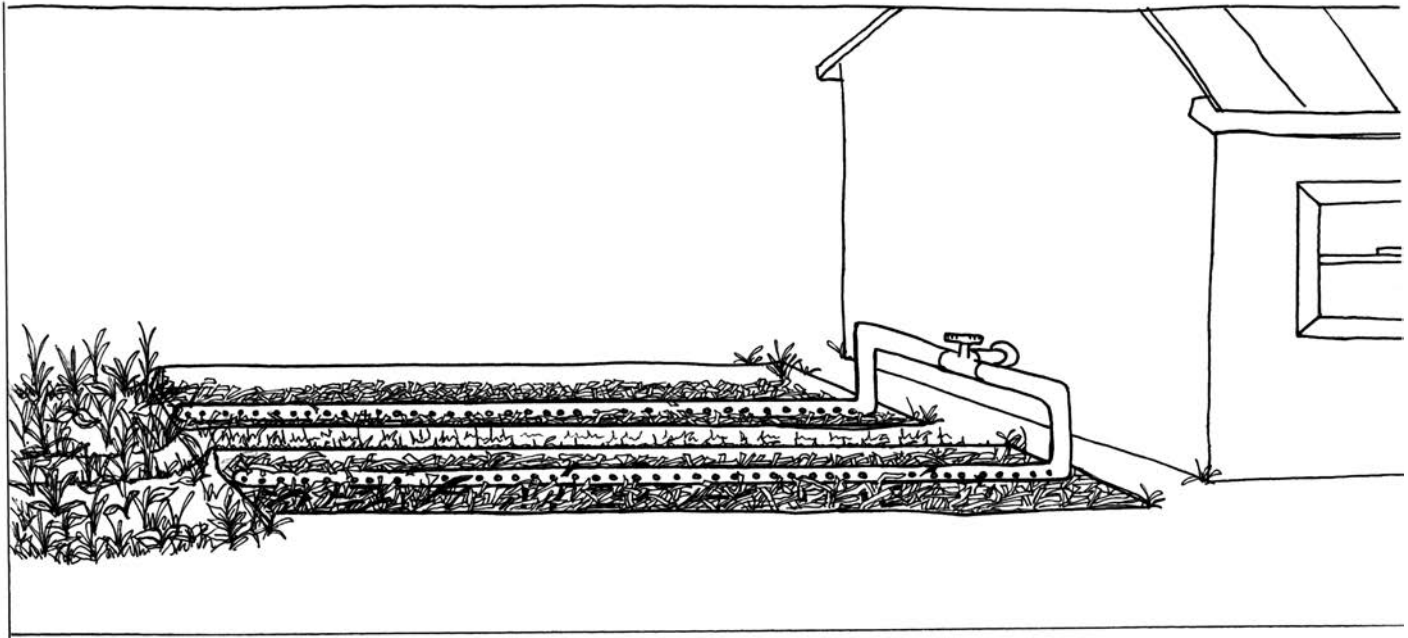
Greywater Trenches, Pattern #48 (See Chapter 6)
