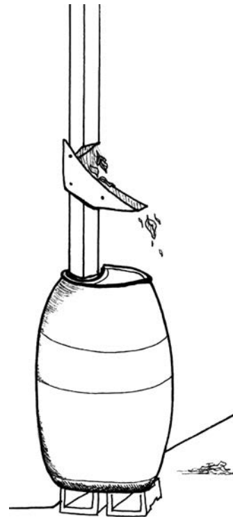
Cutaway downspouts are a commercial item or can be homemade. [Credit: Abi Mustapha]
